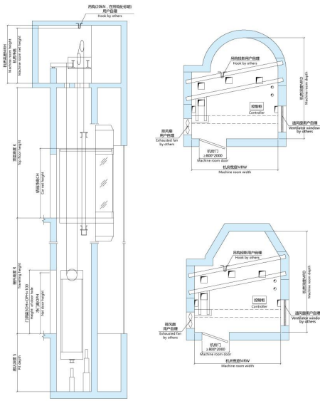
井道立面图 Hoistway elevational drawing
